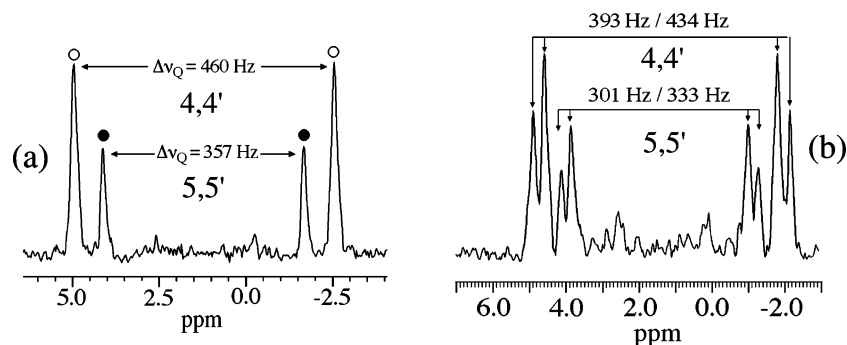
Figure 3. Quadrupolar doublets associated with deuterons 4,4' and 5,5' (sum of columns) extracted from the NAD Q -COSY 2D map of 1 dissolved in (a) the PBLG/ \text{CHCl}_3 achiral phase and (b) the PBLG/ \text{CHCl}_3 chiral phase (see ref 15 for experimental details). The quadrupolar splitting, \Delta\nu_Q , between both components is equal to (3/2)e^2 \times Q_D \times q_{C-D} \times S_{C-D} where Q_D is the deuterium quadrupole moment, q_{C-D} is the electric field gradient (EFG) along the \text{C}-^2\text{H} bond, and S_{C-D} is the order parameter of the \text{C}-^2\text{H} bond.
